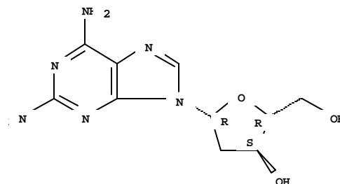
2-Amino-2'-Deoxyadenosine [CAS# 4546-70-7] C 10 H 14 N 6 O 3
