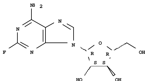
2-Fluoro-9-Arabinoadenine ("Fludarabine") [CAS# 21679-14-1] C 10 H 12 F N 5 O 4
