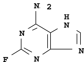
2-Fluoroadenine 98% [CAS# 700-49-2] C 5 H 4 F N 5
