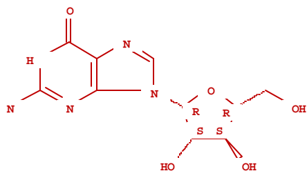
Guanine-9-Arabinoside [CAS# 38819-10-2] C 10 H 13 N 5 O 5
