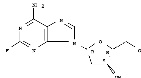
2-Fluoro-2'-Deoxyadenosine [CAS# 21679-12-9] C 10 H 12 F N 5 O 3
