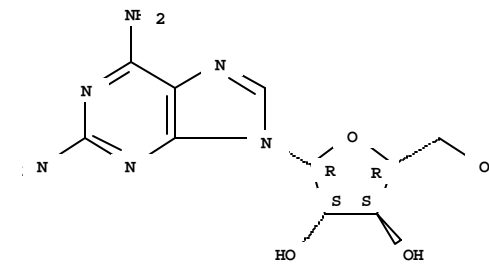
2,6-Diaminopurine arabinoside ( 2-Amino-9-Arabinoadenine ) [CAS# 34079-68-0] C 10 H 14 N 6 O 4
