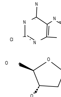
2-Chloro-2'-Deoxyadenosine ("Cladribine") [CAS# 4291-63-8] C 10 H 12 Cl N 5 O 3
