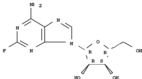
2-Fluoroadenosine 98% [CAS# 146-78-1] C 10 H 12 F N 5 O 4
