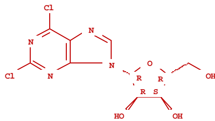
2,6-Dichloropurine-9-Riboside [CAS# 13276-52-3] C 10 H 10 Cl 2 N 4 O 4
